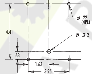
Panel Drilling
